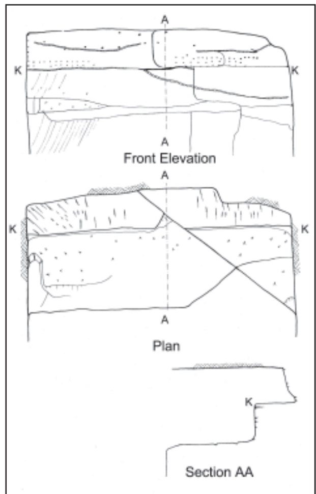
Figure 3: Front elevation, plan and section of the bench showing the chisel marks.
