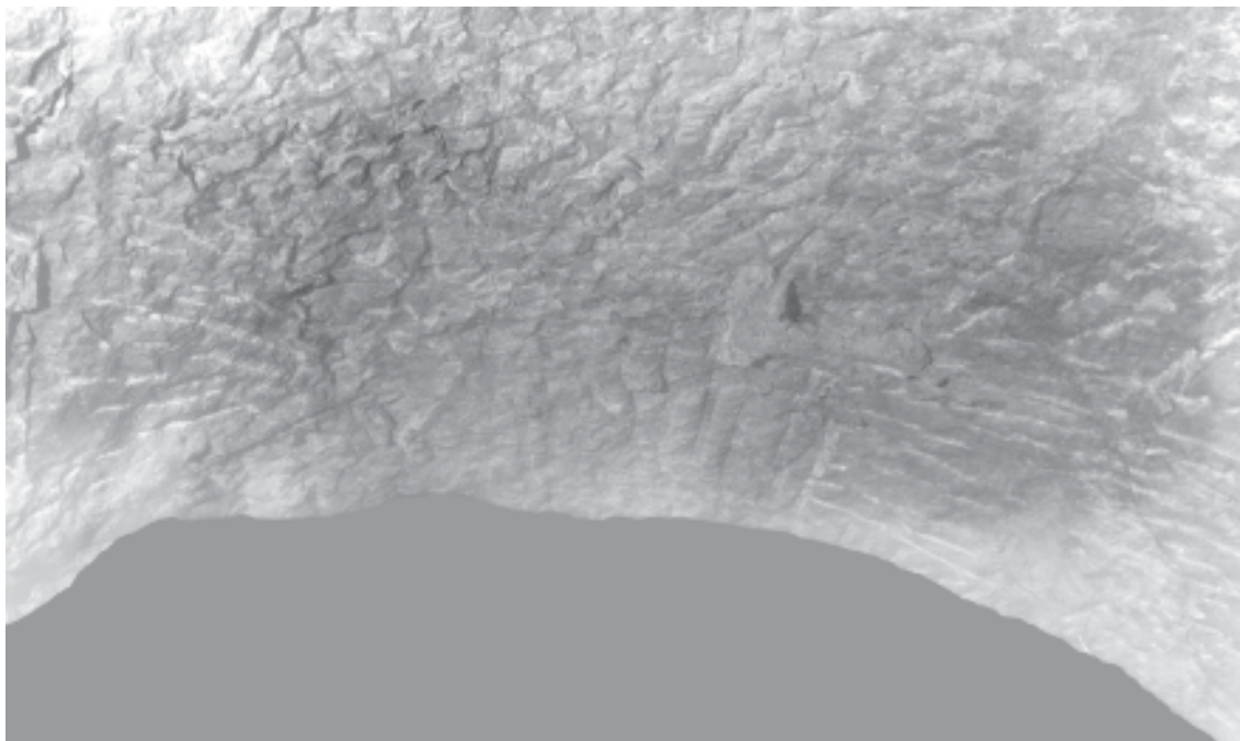
Figure 12: The pattern of chisel marks on the roof of a burial chamber vault. The cone was driven in the centre, and the right side in the photograph (left side of the vault) shows the chisel marks are directed away from the centre of the vault.
